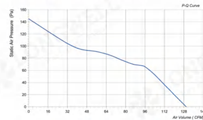
LWDA-100(4")S-PWN-10
