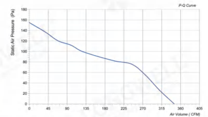
LWDA-150(6")S-PWN-09
