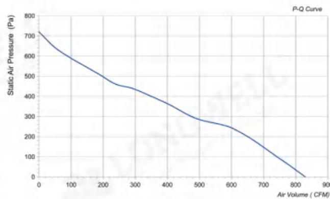
LWDE3G200-IS-05
