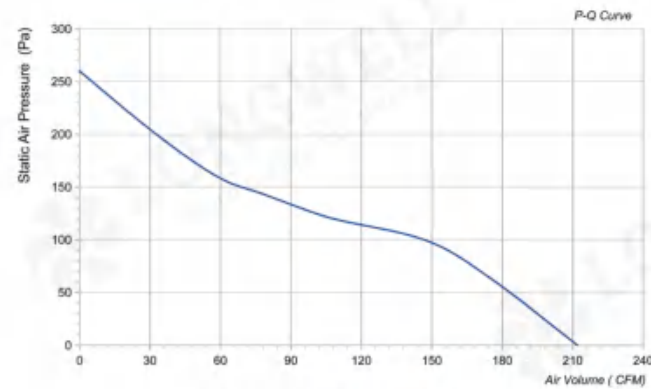
LWDE3G100-IS-05
