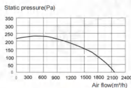
LWDA400S(T)-D02
