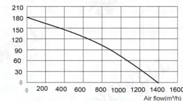
LWDA500S(T)-B02
