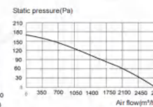
LWDA500S(T)-D02
