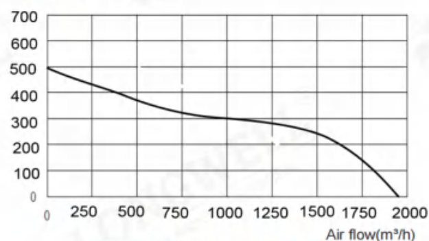
LWDA500S(T)-F03
