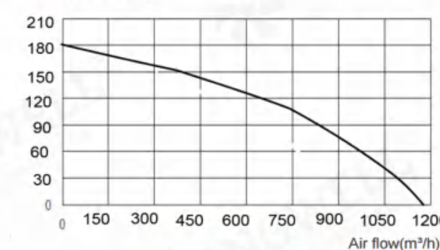
LWDA500S(T)-F02
