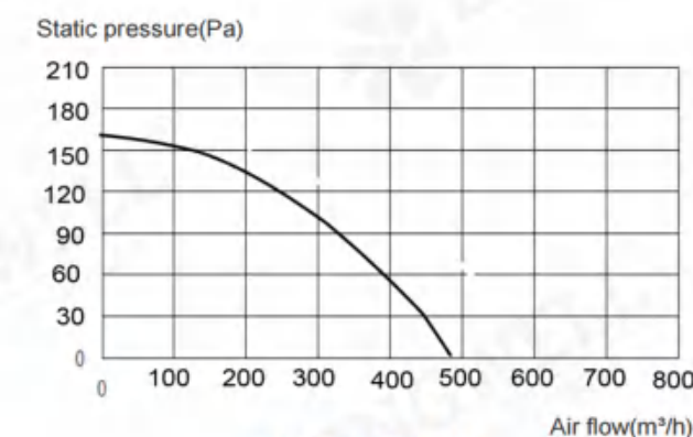
LWDA300S-F02
