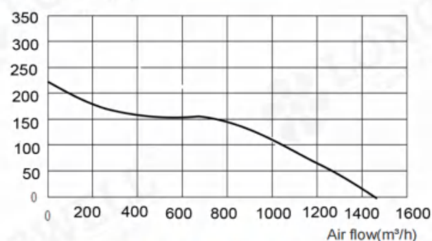
LWDA500S(T)-F04
