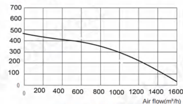
LWDA500S(T)-F01
