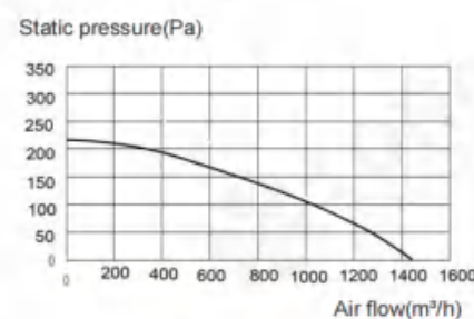
LWDA400S(T)-D03
