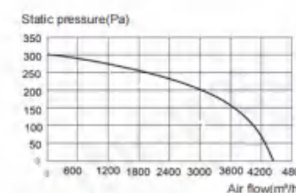
LWDA500S(T)-D01
