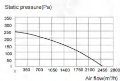
LWDA400S-D01
