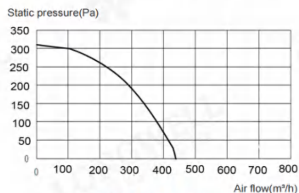
LWDA250S-F01
