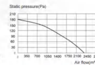
LWDA500S(T)-D04
